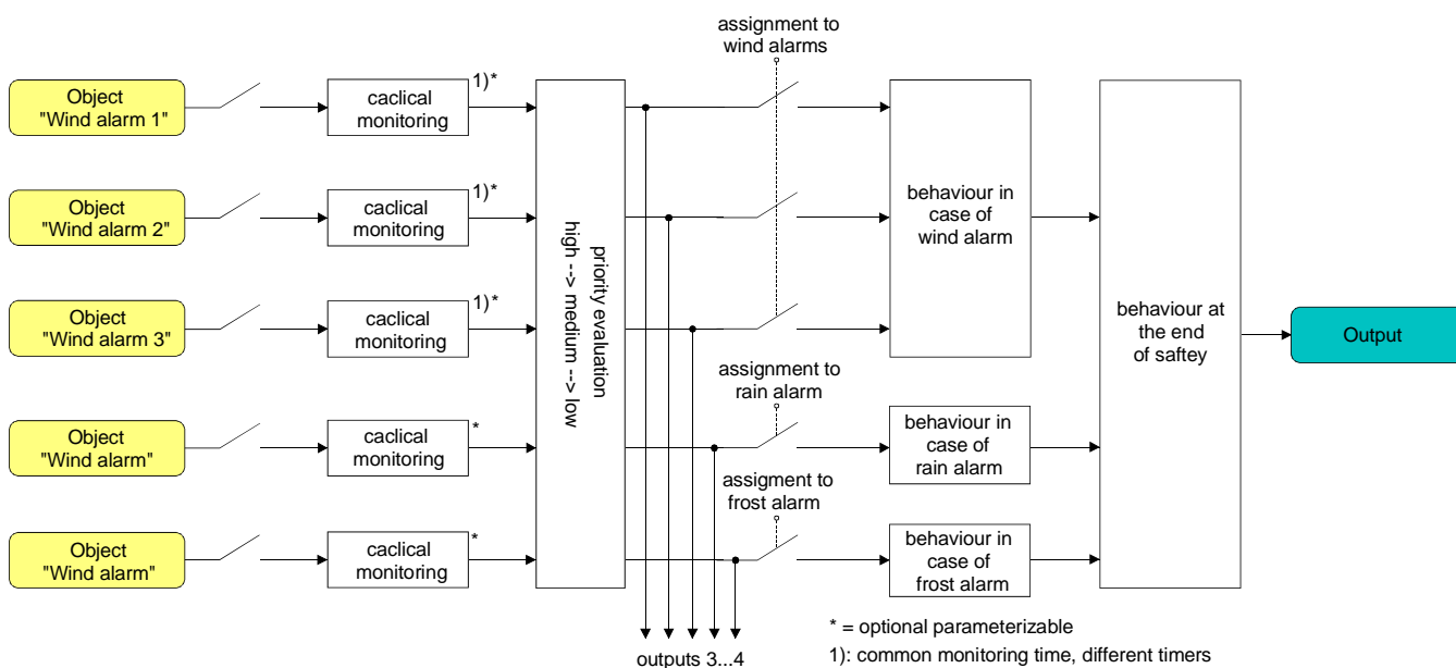
Fig. 16: Function diagram of channel-oriented safety functions
