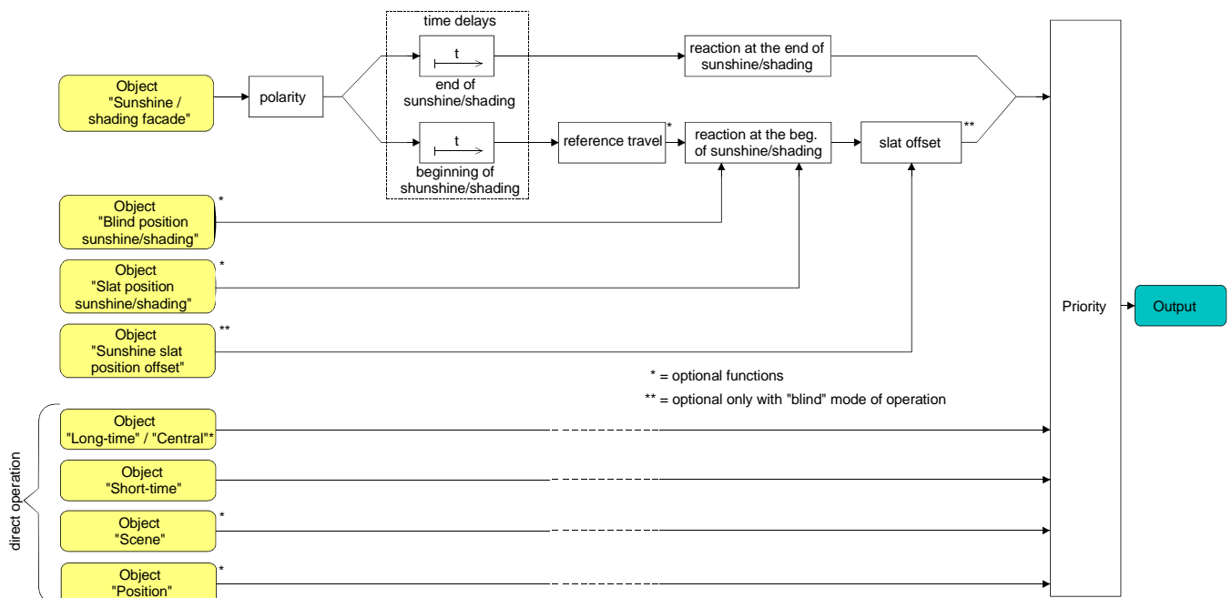
Fig. 19: Function diagram illustrating the simple sun protection
