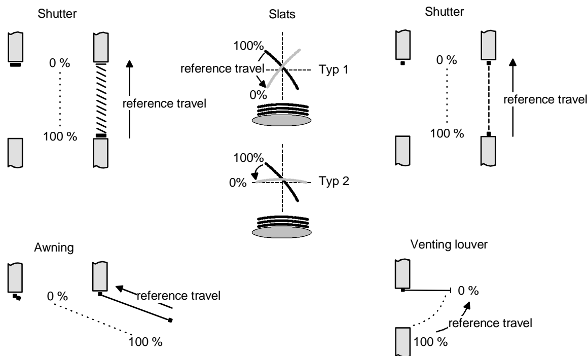
Fig. 15: Reference travel
