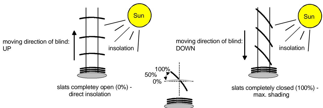
Fig. 11: Type 2 - slatted blinds with oblique and horizontal slat position
