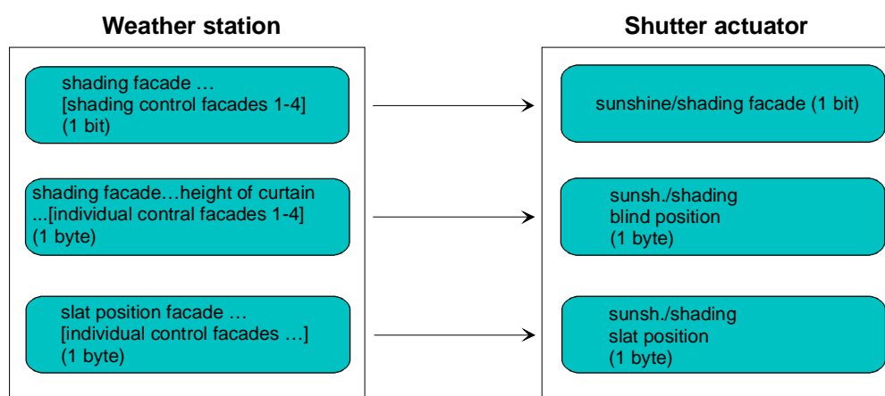
Fig. 26: Programming of the communication objects for application example IV
