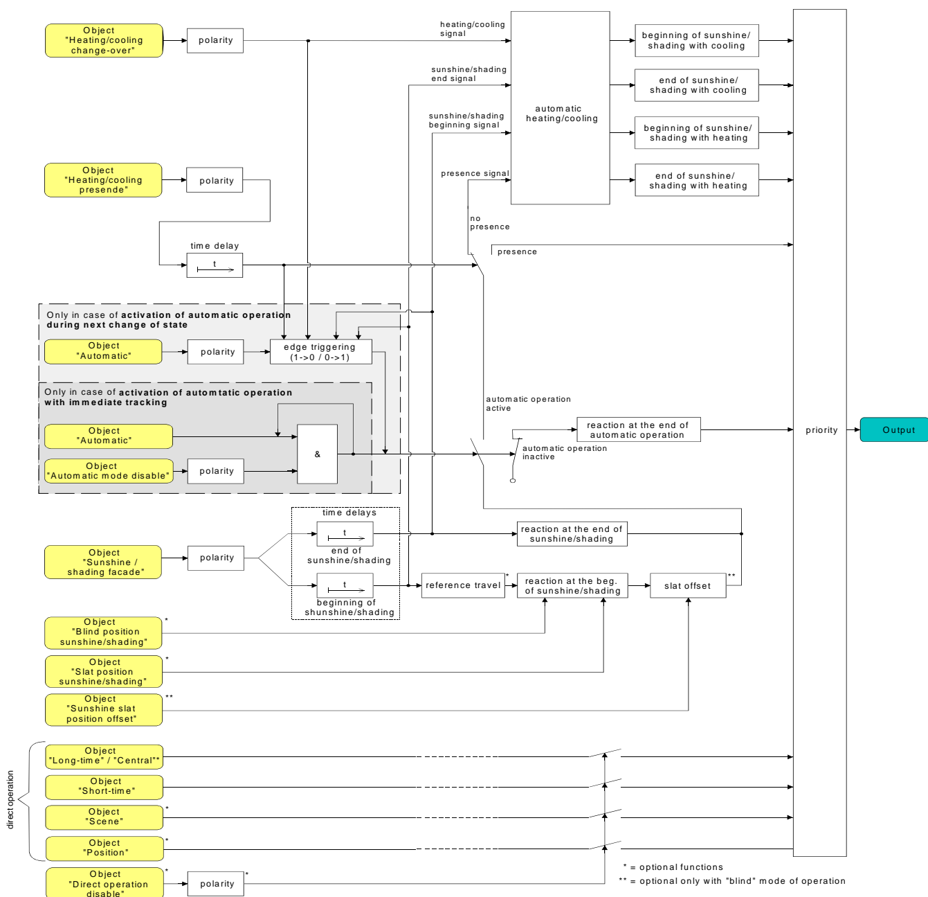
Fig. 29: Schematic diagram of automatic heating/cooling
