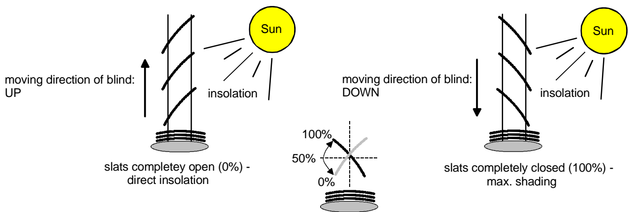
Fig. 10: type 1 - slatted blinds with oblique slat position in both travel directions
