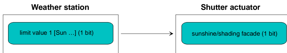
Fig. 23: Programming of the communication objects for application example I
