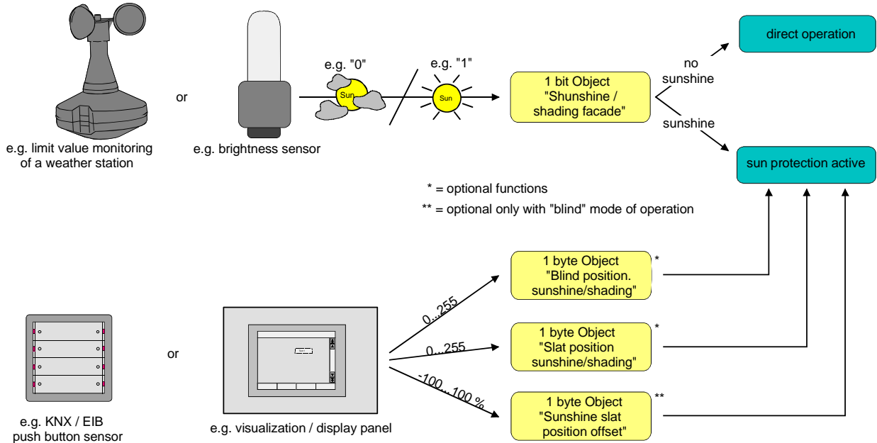
Fig. 18: Schematic diagram illustrating the simple sun protection configuration
