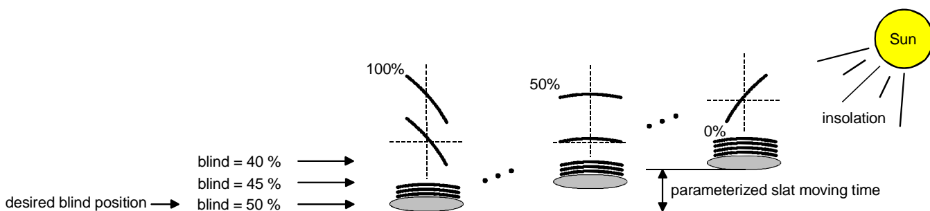
Fig. 13: Example of slat positioning affecting the position of the blind (typical of slat type 1; analogous reaction for type 2)
