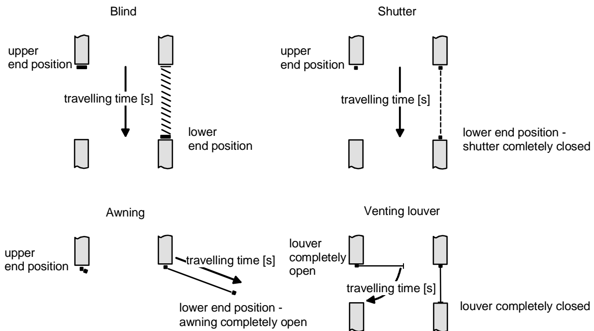
Fig. 9: Travelling time as a function of the type of movement
