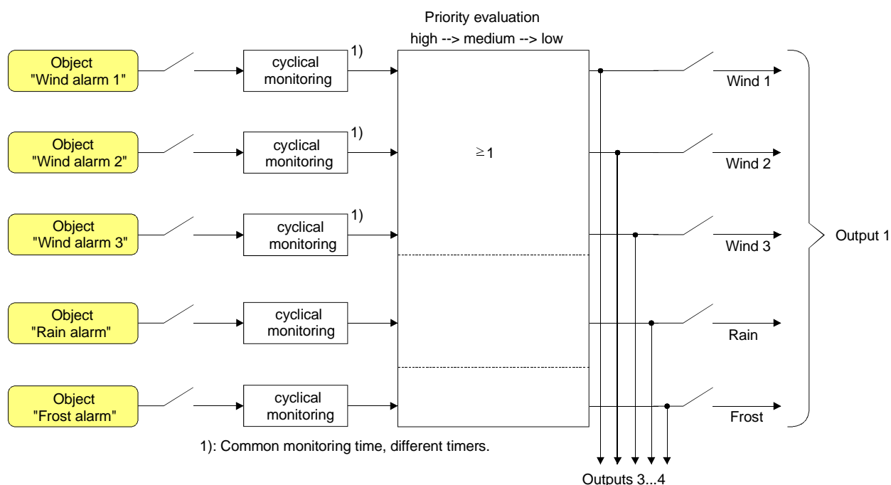
Fig. 8: Function diagram of the safety function
