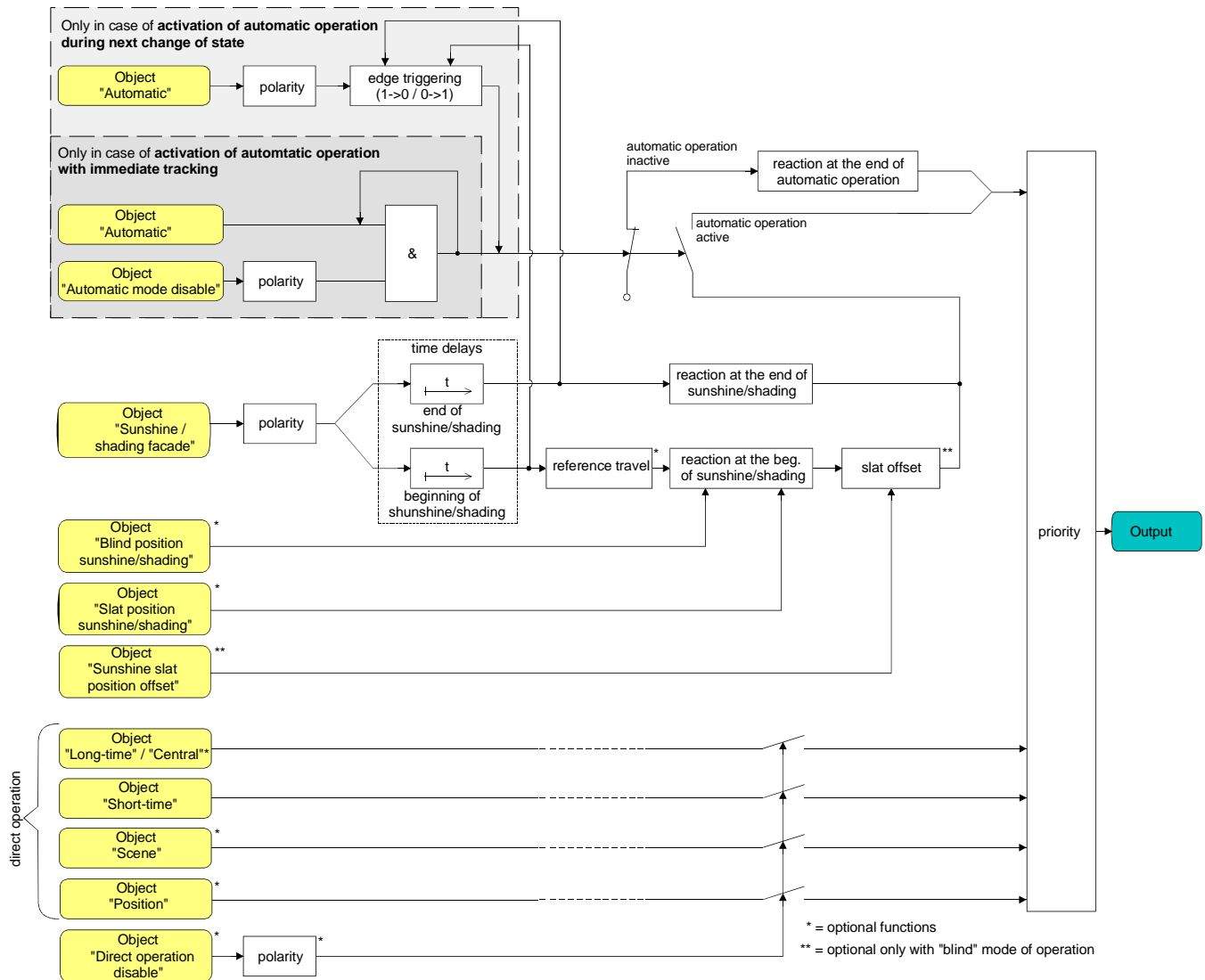
Fig. 21: Functional diagram illustrating the enlarged sun protection
