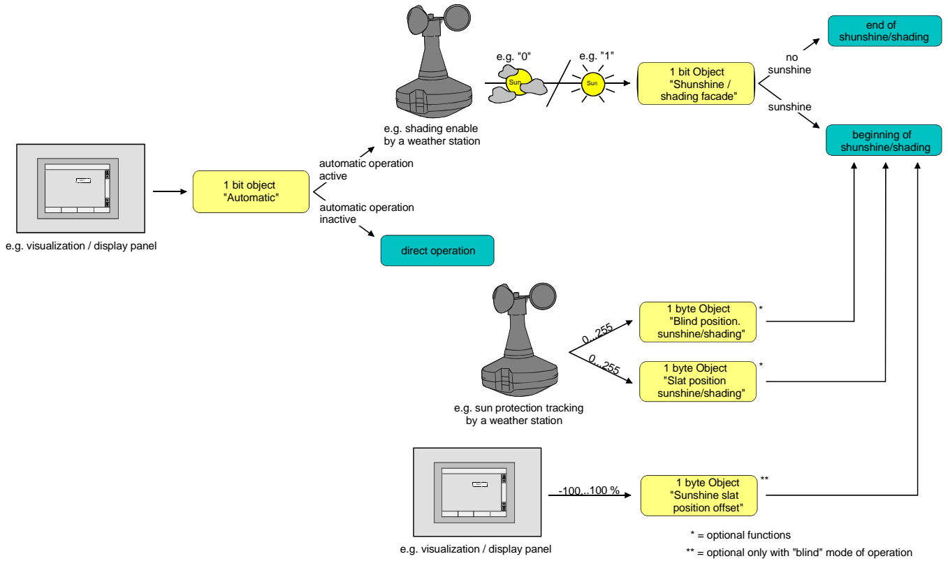
Fig. 20: Schematic diagram illustrating the enlarged sun protection configuration (for reasons of simplicity without disabling functions)
