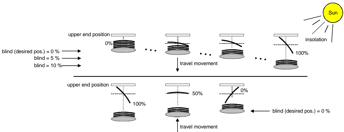
Fig. 14: Example of slat positioning with the blind in upper end position (typical of slat type 1)
