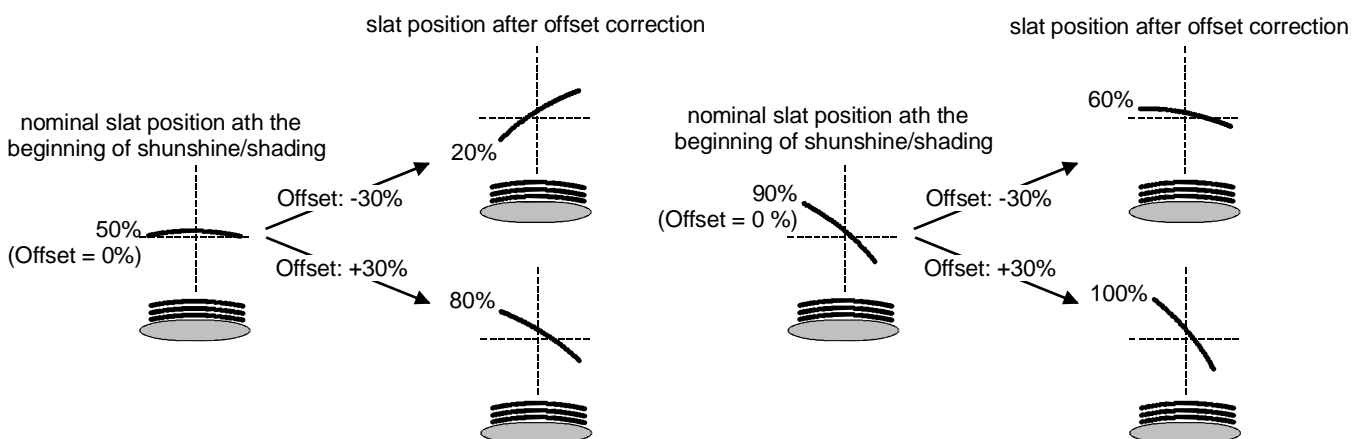
Fig. 22: Functional principle of slat offset (example showing slat type 1 / slat type 2 identical)
