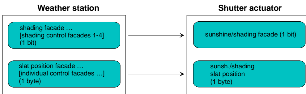
Fig. 25: Programming of the communication objects for application example III
