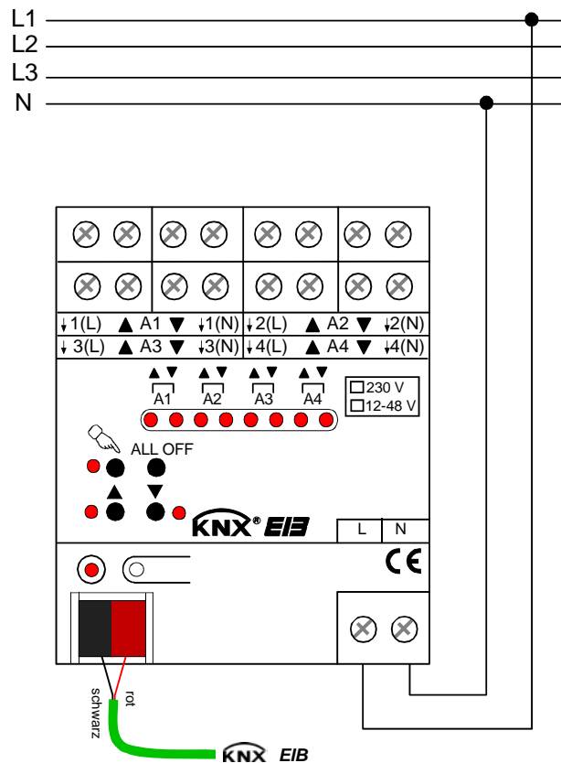
Fig. 1: Electrical connection of mains voltage
