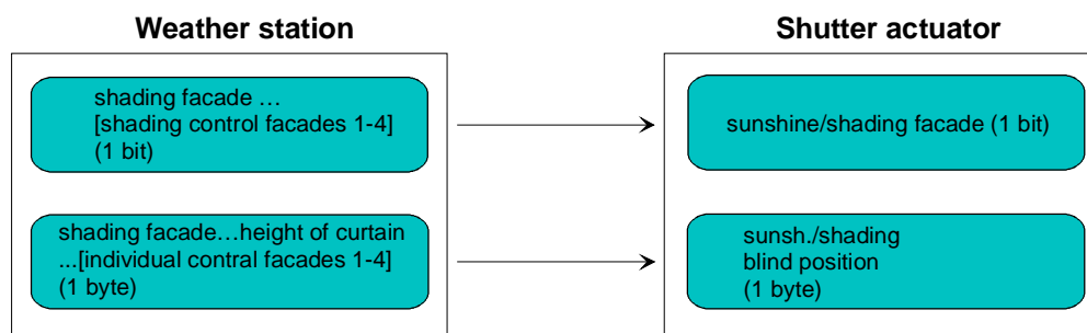
Fig. 27: Programming of the communication objects for application example V
