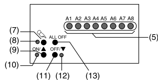
Fig.2: Controls – layout
