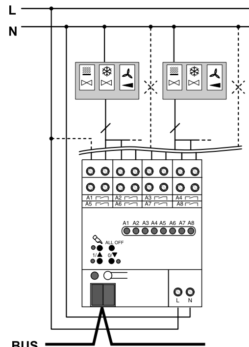
Fig. 6: connection of the load for 2 fan coil outputs
